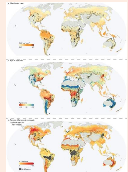
Figure 27. Carbon removal potential of secondary forests (Robinson et al. Preprint). The maps show (a) maximum rate possible over the first 100 years of stand growth, (b) age at which the maximum is achieved, and (c) places where older secondary forests can remove substantially more carbon than brand new regrowth
