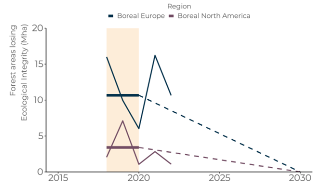
Figure 19. Net area of forests that transitioned to a lower integrity class in boreal regions from 2018-2022, in million hectares (Mha)
