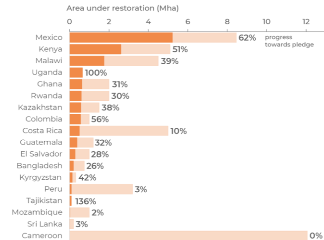
Figure 24. Country pledges under the Bonn Challenge and progress reported up to 2022 through the Restoration Barometer, in million hectares (Mha). The light orange bars represent countries' pledges, and the dark orange bars represent the progress reported by countries
