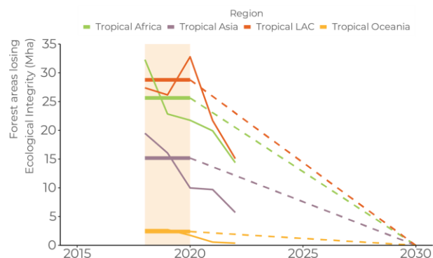
Figure 17. Net area of forests that transitioned to a lower integrity class in tropical regions from 2018-2022, in million hectares (Mha)
