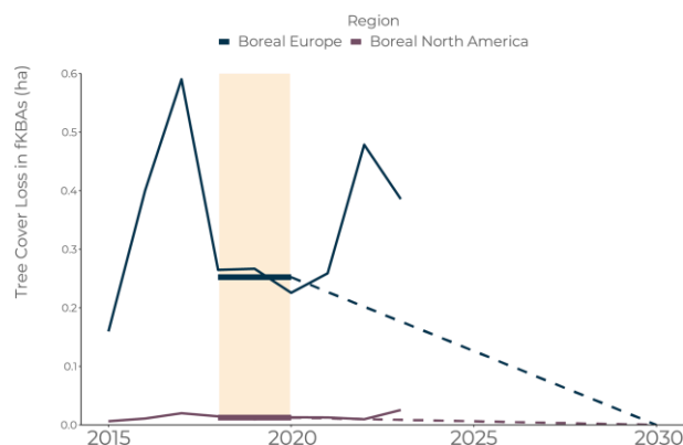
Figure 37. Boreal tree cover loss in forested KBAs (fKBAs) from 2015-2023, in hectares (ha)
