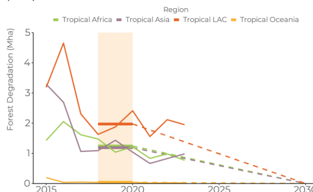
Figure 14. Degradation of tropical moist forests from 2015-2023, in millions of hectares (Mha)
