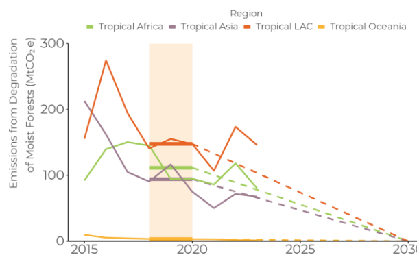
Figure 15. Emissions from the degradation of tropical moist forests at the regional level from 2015-2023, in million metric tons of carbon dioxide equivalent (MtCO 2 e)
