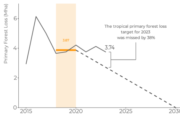
Figure 8. Global (pantropic) primary forest loss from 2015-2023, in millions of hectares (Mha) and additional key metrics
