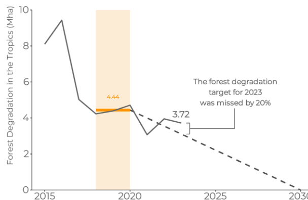
Figure 12. Degradation of tropical moist forests from 2015-2023, in millions of hectares (Mha)
