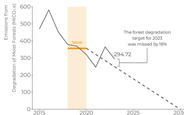
Figure 13. Emissions from the degradation of tropical moist forests from 2015-2023, in million metric tons of carbon dioxide equivalent (MtCO 2 e)
