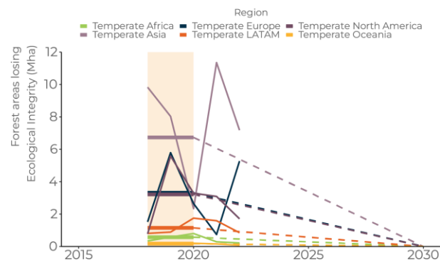
Figure 18. Net area of forests that transitioned to a lower integrity class in temperate regions from 2018-2022, in million hectares (Mha)
