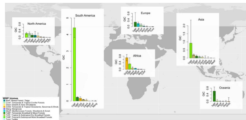
Figure 33: Total additionally preserved above-ground carbon (AGC) aggregated by continent and biome
