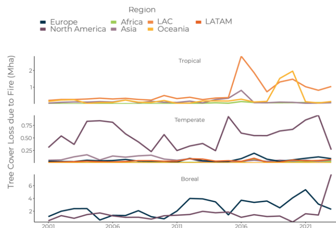
Figure 21. Tree cover loss due to fires from 2001-2023 in million hectares (Mha)
