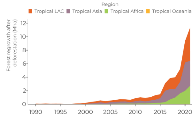
Figure 26. Global tropical moist forest regrowth after deforestation from 1990-2021, in million hectares (Mha)
