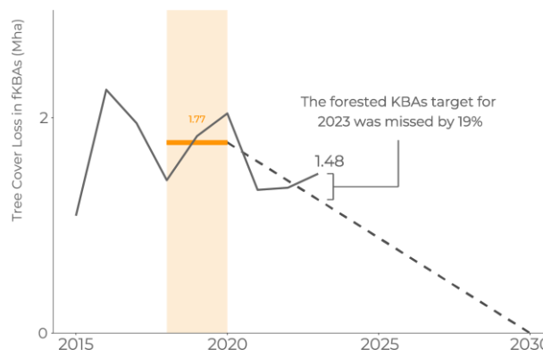
Figure 34. Global tree cover loss in forested KBAs (fKBAs) from 2015-2023, in million hectares (Mha)
