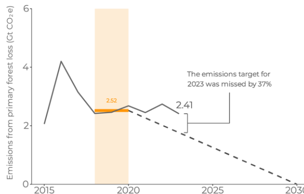
Figure 9. Emissions from primary forest loss from 2015-2023, in billions of metric tons of carbon dioxide equivalent (GtCO 2 e) and additional key metrics
